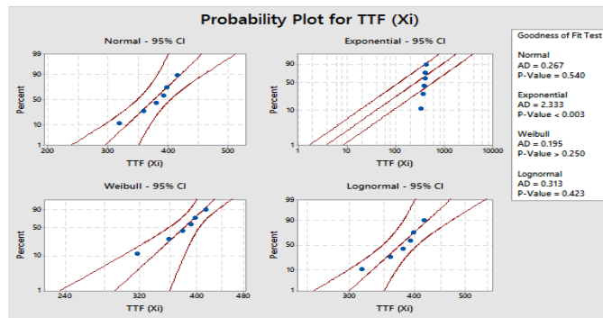
Gambar 3. Uji Goodness of fit TTF Hose
