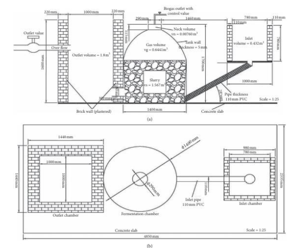
FIGURE 4: Schematic layout of the designed biogas digester system showing the front and above view. (a) View of the fabricated digester from front. (b) View of the fabricated digester from above.
