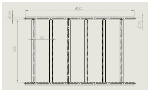
Gambar 2. Alat penelitian Heat Exchanger panjang tube 500 mm 12 belokan
