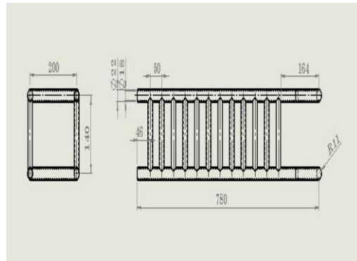
Gambar 4. Alat penelitian Heat Exchanger panjang tube 125 mm 48 belokan
