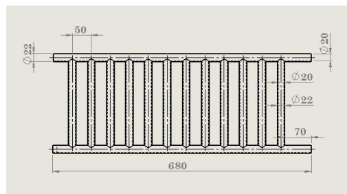
Gambar 3. Alat penelitian Heat Exchanger panjang tube 250 mm 24 belokan
