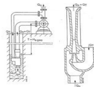
Gambar 6. Jet Pumps.
