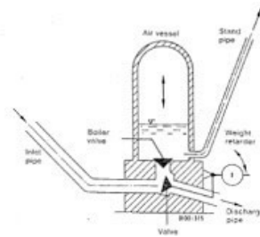
Gambar 8. Hydraulic Rams
