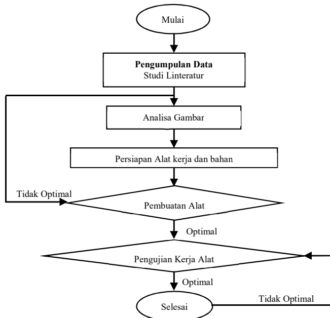
Gambar 10. Flowchat Penelitian
