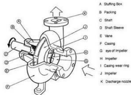
Gambar 1. Pompa Sentrifugal ( Centrifugal Pump )
