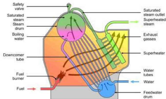
Gambar 2. Boiler pipa air (Sumber: Yendri, 2011)
