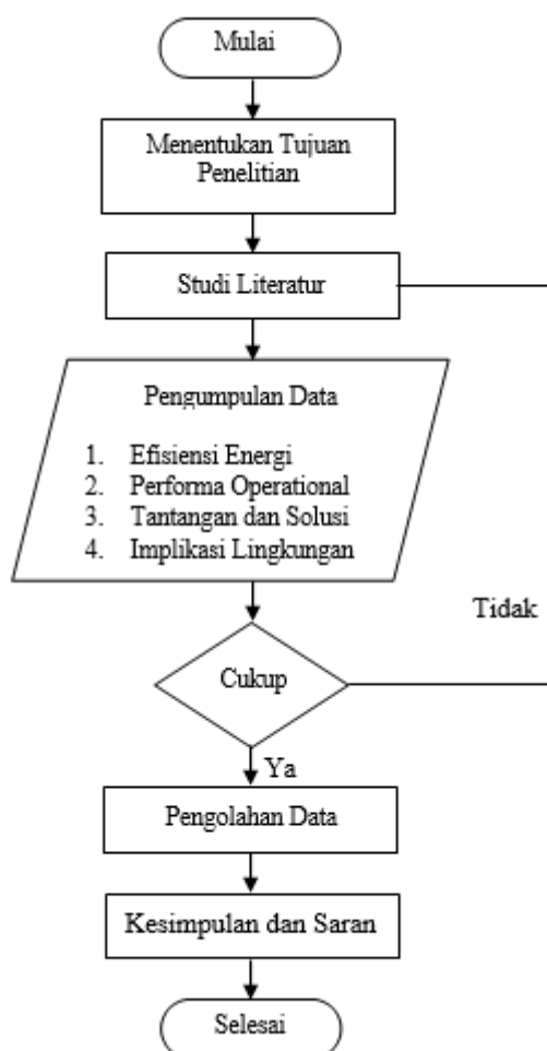
Gambar 2 Flowchart Penelitian
