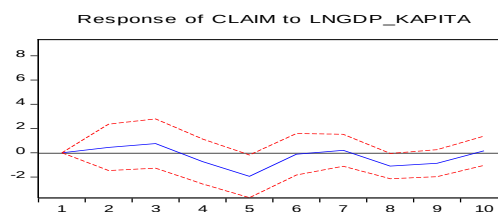
Response to Cholesky One S.D. (d.f. adjusted) Innovations \pm 2 S.E.
